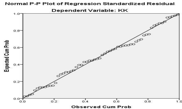
Figure 2. PP Plot Normality Test
