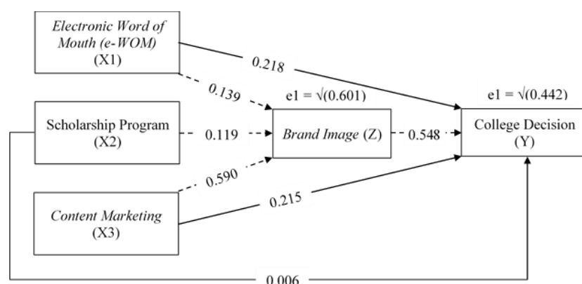
Figure 2. Path Diagram Model 2
