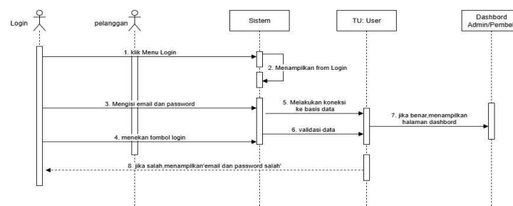
Figure 5. Login Sequence Diagram
