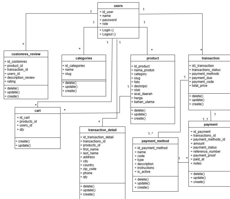
Figure 8. Class Diagram
