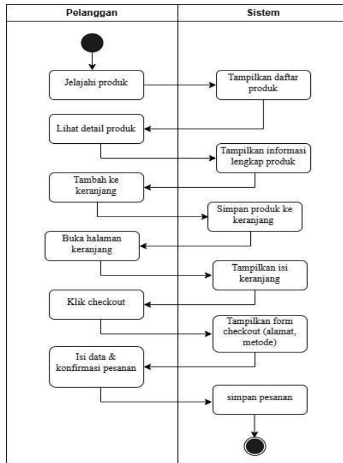
Figure 3. Ordering Activity Diagram
