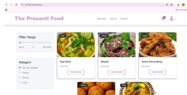
Figure 14. Shopping Page
