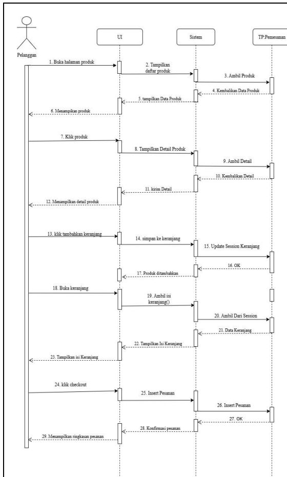
Figure 6. Ordering Sequence Diagram
