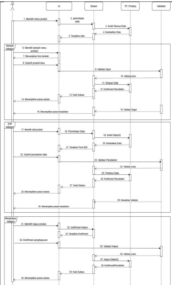
Figure 7. Sequence Diagram for Managing Products
